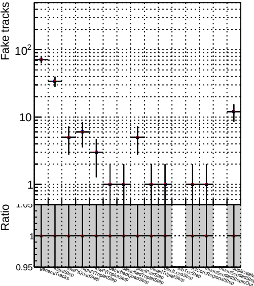
Number ● DQM_V0001_R0000000001_Global_CMSSW_mkt50i5_RECO ★ DQM_V0001_R0000000001_Global_CMSSW_mkt50i6_RECO
