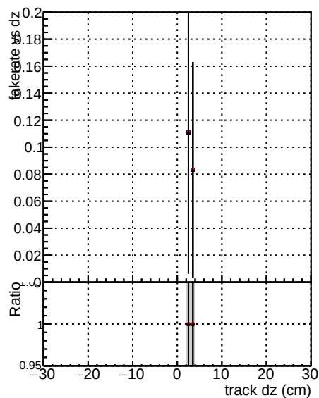
DOM V0001 DOM V0001 DOM V0001 Global Global Global CMSSW mkt5014 RECO CMSSW mkt5014 RECO CMSSW mkt5014 RECO Fake rate vs d
