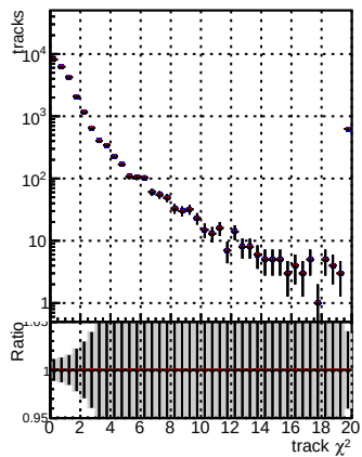
N of reco track vs. BOM V0001 R0000000001 Global CMSSW mkt5014 RECO BOM V0001 R0000000001 Global CMSSW mkt5016 RECO
