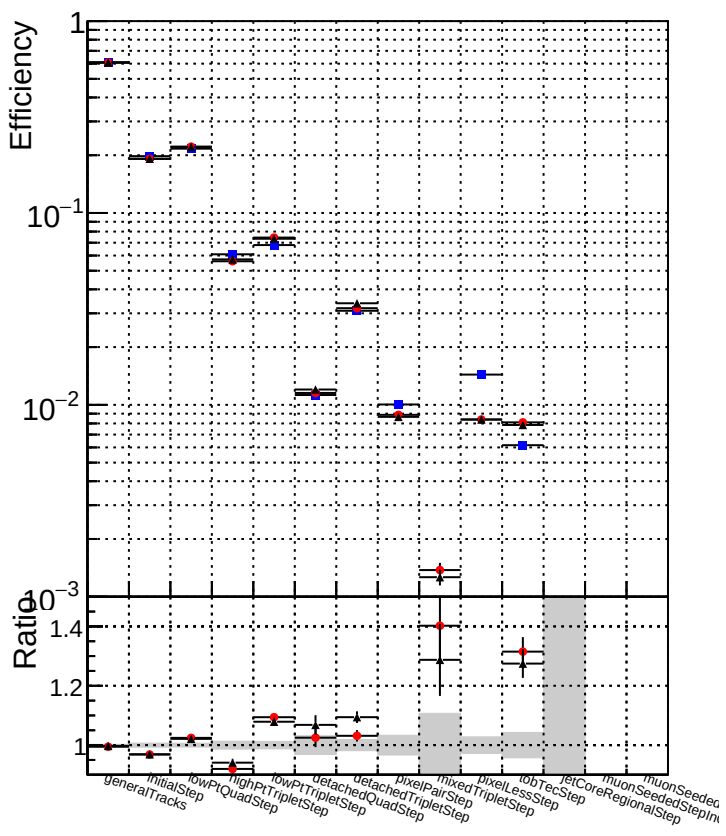
DQM_CKF_TTbarPU DQM_mkFit_TTbarPU-noDNN-baseline DQM_mkFit_TTbarPU-noDNN-fix
