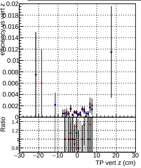
Efficiency vs TP vert z (cm) Legend: DQM_CKF_TTbarPU DQM_mkFit_TTbarPU-noDNN-baseline DQM_mkFit_TTbarPU-noDNN-fix
