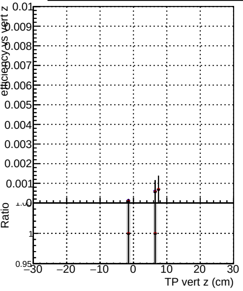
Efficiency vs vertpos DQM_CKF_TTbarPU DQM_mkFit_TTbarPU-noDNN-baseline DQM_mkFit_TTbarPU-noDNN-fix
