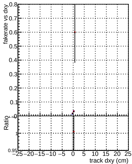
—•— DOM CKE TTbarPU —•— BOM mkttt TTbarPU-noBNN-baseline —•— BOM mkttt TTbarPU-noBNN-fix
