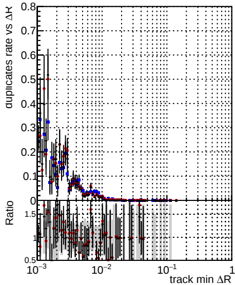
Legend: \blacksquare DOM_CKF_TTbarPU \bullet DOM_mkFit_TTbarPU-noDNN-baseline \times DOM_mkFit_TTbarPU-noDNN-fix
