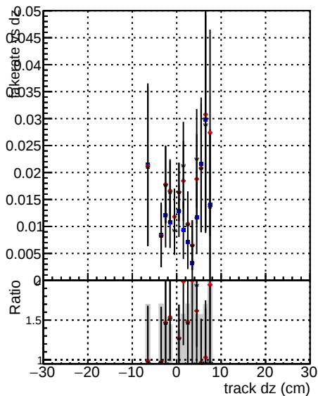
—•— DOM CKF TTbarPU —•— BOM-mkFit TTbarPU-noBNN-fix Ratio
