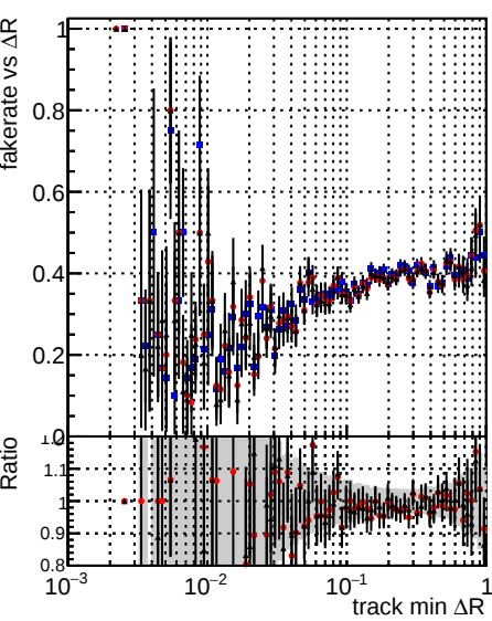
Legend: DQM_CKF_TTbarPU (black circles), DQM_mkFit_TTbarPU-noDNN-baseline (red circles), DQM_mkFit_TTbarPU-noDNN-fix (blue circles)
