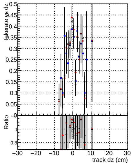
Fake rate vs dz Legend: DOM CKE TTbarPU (black line) DOM mktFit TTbarPU-noBNN-baseline (red line) DOM mktFit TTbarPU-noBNN-fix (blue line)
