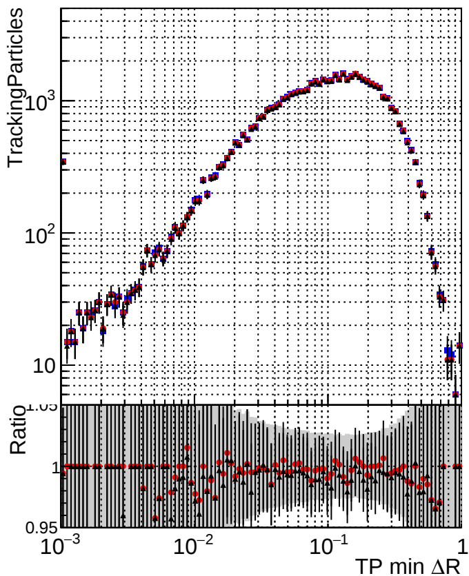
N of simulated tracks vs \Delta R(\text{TP, jet})
