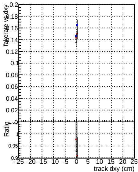
—•— DOM CKF TTbarPU —•— DOM mktT TTbarPU-noBNN-bx —•— DOM mktT TTbarPU-noBNN-fix
