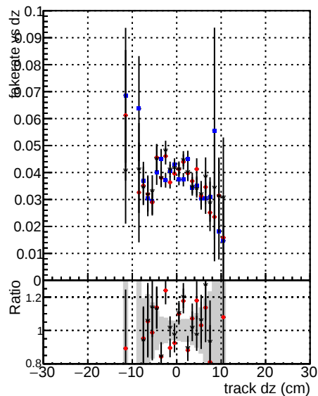
Fake rate vs dz DOM CKE TTbarPU DOM mkttt TTbarPU-noBNN-fix baseline
