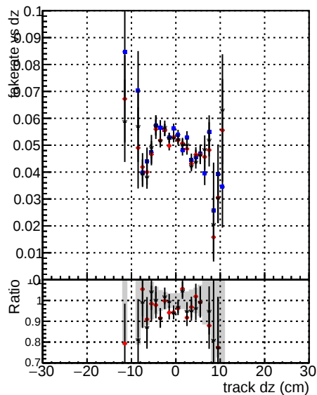
— DOM CKF TTbarPU — BQM mktFit TTbarPU-noBNN-baseline
