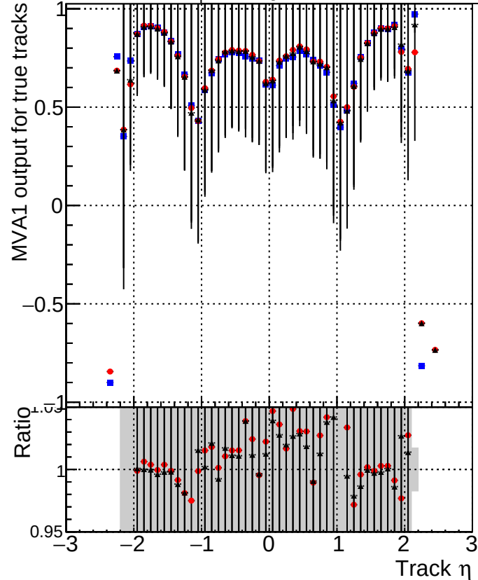
MVA1 of associated tracks (recoToSim) vs. track \eta Legend: ■ DQM_CKF_TTbarPU ● DQM_mkFit_TTbarPU-noDNN-baseline ★ DQM_mkFit_TTbarPU-noDNN-fix
