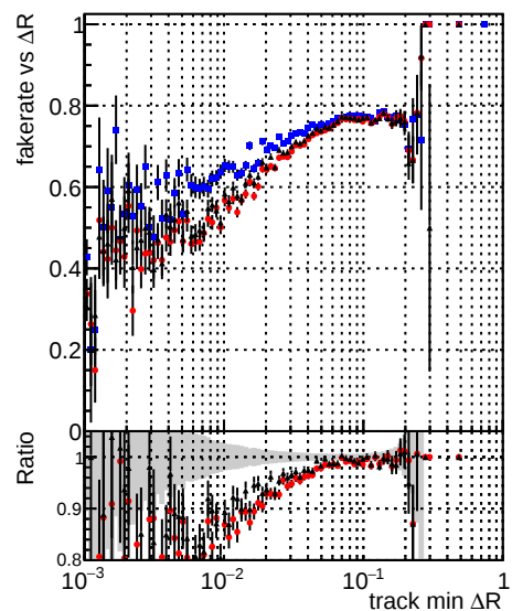
Fake rate vs \Delta R(\text{track, jet}) DQM_CKF_TTbarPU DQM_mkFit_TTbarPU-noDNN-baseline DQM_mkFit_TTbarPU-noDNN-fix
