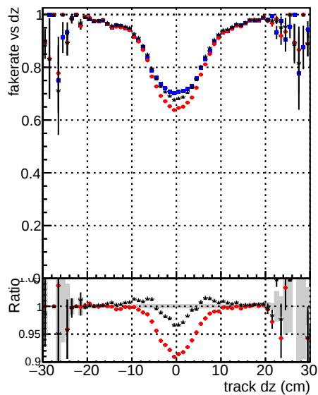
Legend: DOM CKF TTbar PU Fake rate vs d DOM mktFit TTbarPU-noBNN-baseline
