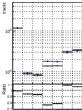
N of reco track vs. s Legend Model Blue square DOM CRF T1barPU Red dot DOM mkFit T1barPU-noDNN-baseline Black dot DOM mkFit T1barPU-noDNN-fix
