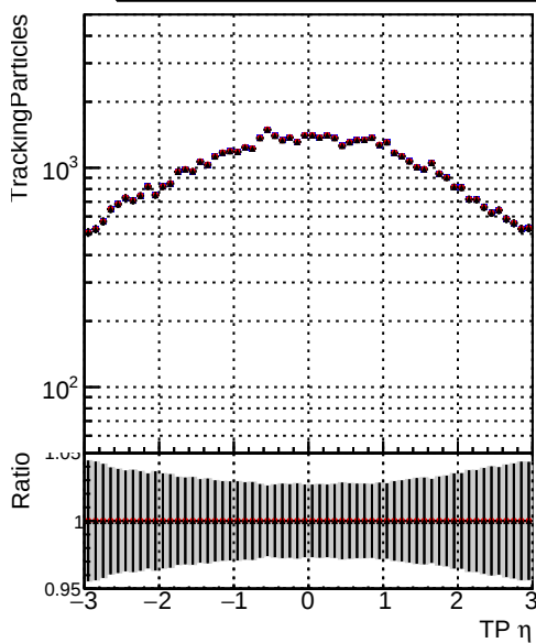
—•— DQM_CKF_TTbarPU —•— DQM_mkFit_TTbarPU-noDNN-baseline —•— DQM_mkFit_TTbarPU-noDNN-fix
