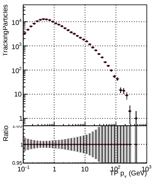
—•— DQM_CKF_TTbarPU —•— DQM_mkFit_TTbarPU-noDNN-baseline —•— DQM_mkFit_TTbarPU-noDNN-fix
