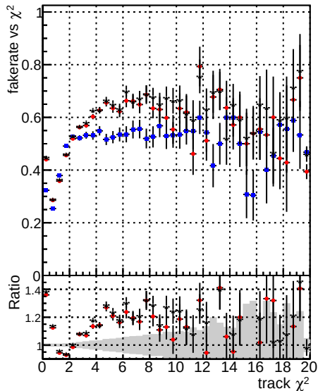
Fake rate vs. — DOM CKF TTbarPU — DOM mkt TTbarPU-noBNN-baseline
