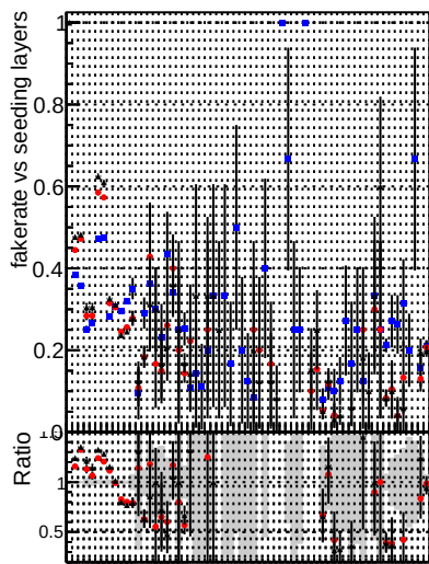
Fake rate vs. — DOM CKF TTbarPU — DOM mkt TTbarPU-noBNN-baseline
