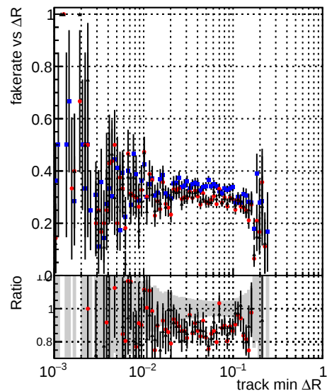
Legend: DQM_CKF_TTbarPU (black line with dots) DQM_mkFit_TTbarPU-noDNN-baseline (red line with dots) DQM_mkFit_TTbarPU-noDNN-fix (blue line with dots)
