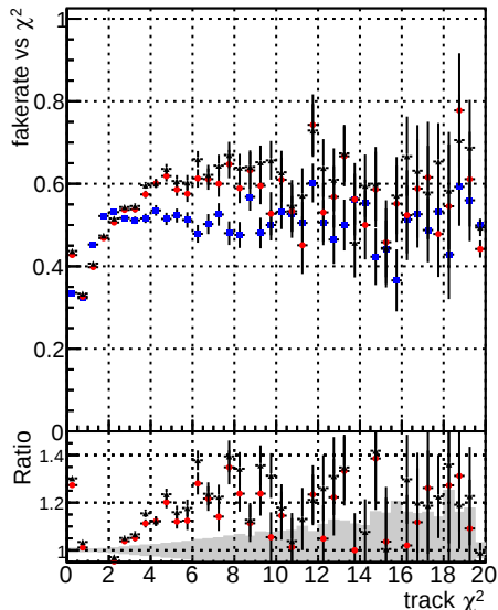
Fake rate vs. DOM CKF TTbarPU BOM mktf TTbarPU-noBNN-baseline
