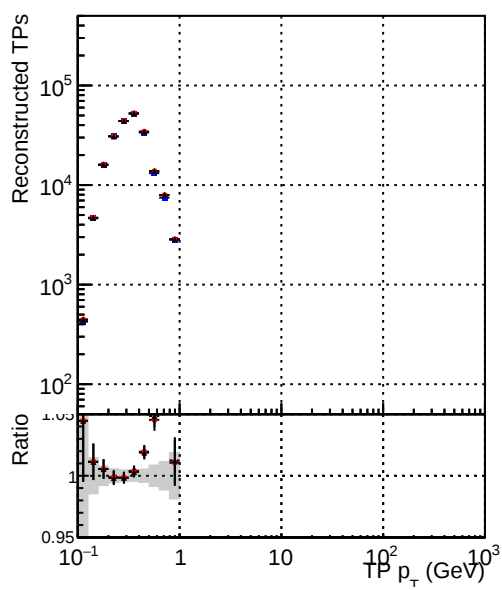
Legend: DQM_CKF_SoftQCD (blue circles), DQM_mkFit_SoftQCD-noDNN-baseline (red circles), DQM_mkFit_SoftQCD-noDNN-fix (black circles)
