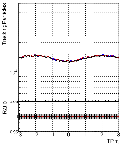
Legend: DQM_CKF_SoftQCD (blue circles), DQM_mkFit_SoftQCD-noDNN-baseline (red circles), DQM_mkFit_SoftQCD-noDNN-fix (black circles)
