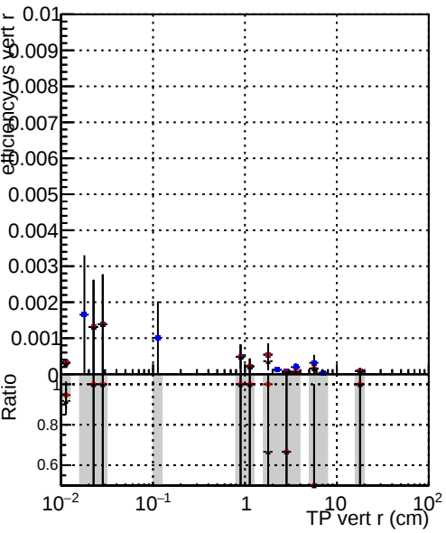
Efficiency vs vertpos DQM_CKF_SoftQCD DQM_mkFit_SoftQCD-noDNN-baseline DQM_mkFit_SoftQCD-noDNN-fix
