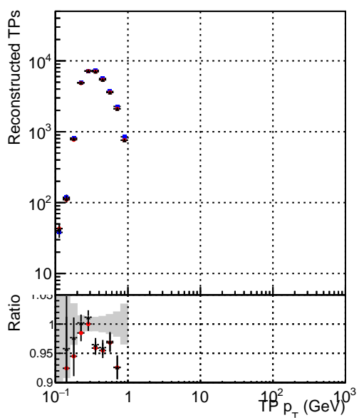
Legend: DQM_CKF_SoftQCD (blue dots), DQM_mkFit_SoftQCD-noDNN-baseline (red dots), DQM_mkFit_SoftQCD-noDNN-fix (black dots)
