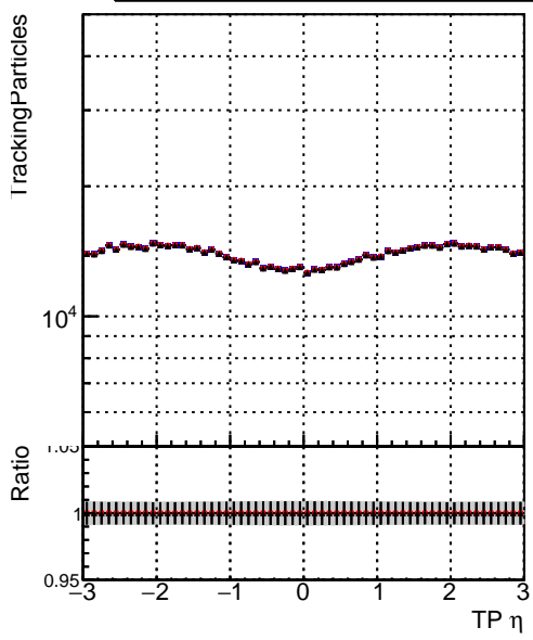
Legend: DQM_CKF_SoftQCD (blue dots), DQM_mkFit_SoftQCD-noDNN-baseline (red dots), DQM_mkFit_SoftQCD-noDNN-fix (black dots)
