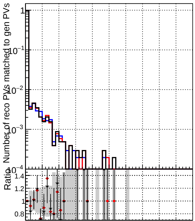
RecoPVAssoc2GenPVMatched_missing
