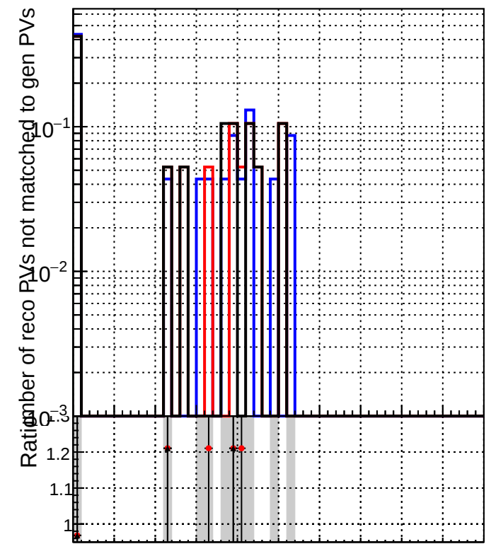
RecoPVAssoc2GenPVNotMatched_missing
