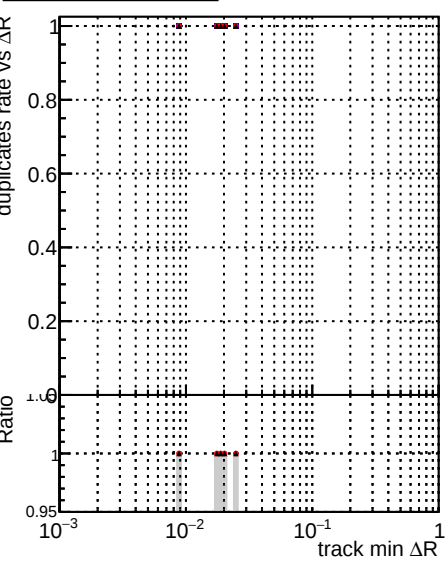
DOM_CKF_SoftQCD, DOM_mkFit_SoftQCD-noDNN-baseline, DOM_mkFit_SoftQCD-noDNN-fix
