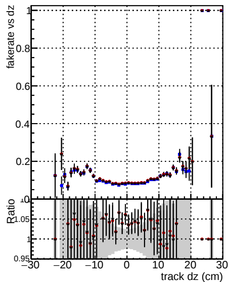
Fake rate vs dz Legend: DOM CKF SoftQCD DOM CKF SoftQCD-noBNN-baseline DOM CKF SoftQCD-noBNN-fix
