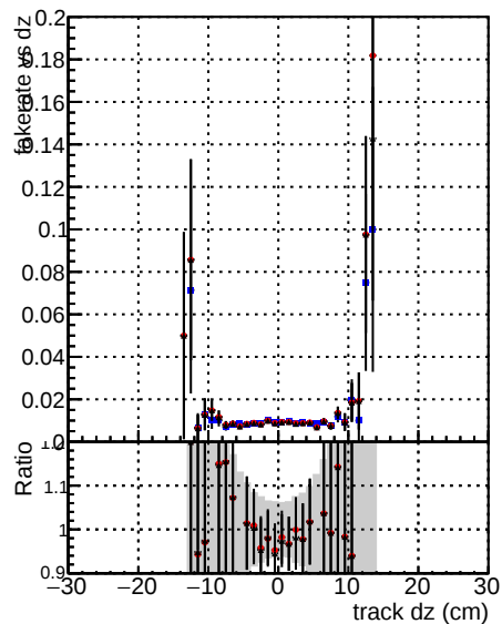
Fake rate vs dz —•— DOM CKF SoftOCB —•— DOM CKF SoftOCB-noDNN-baseline —•— DOM mktFit SoftOCB-noDNN-fix
