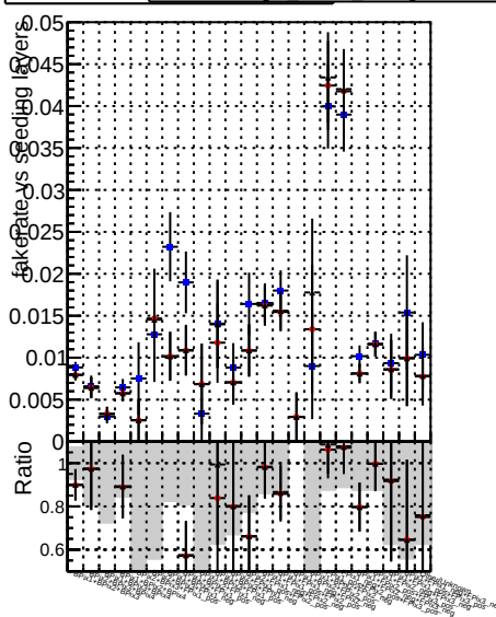
Fake rate vs. DOM CKF SoftOCB BOM mkt SoftOCB-noBNN-fix baseline
