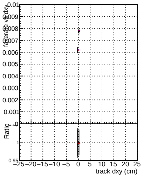
Fake rate vs d DOM CKF SoftQCD DOM CKF SoftQCD-noBNN-baseline DOM CKF SoftQCD-noBNN-fix
