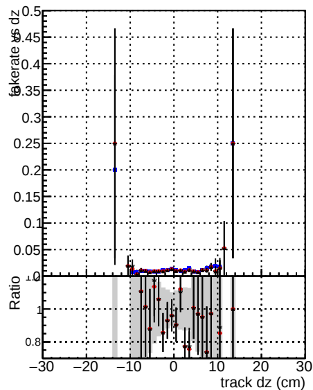
Legend for Fake rate vs d, Duplicates Rate vs Dxy, and Pileup rate vs dxy plots: DOM CKF (blue dots) SoftOCB (red dots) DOM mktFit (black dots) SoftOCB-noBNN-fix (grey dots)
