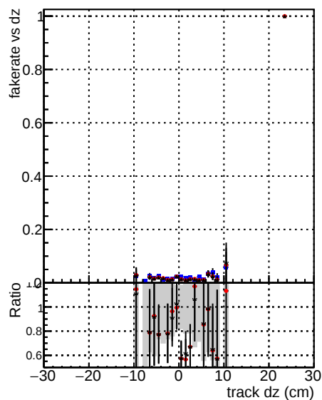
Fake rate vs dz — DOM CKE SoftOCB — DOM mktFit SoftOCB-noBNN-fix
