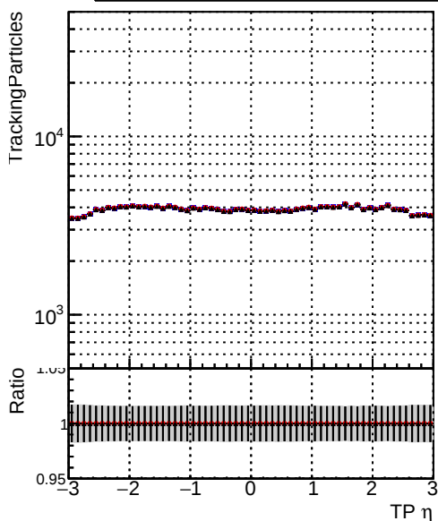
● DQM_CKF_SoftQCD ● DQM_mkFit_SoftQCD-noDNN-baseline ● DQM_mkFit_SoftQCD-noDNN-fix
