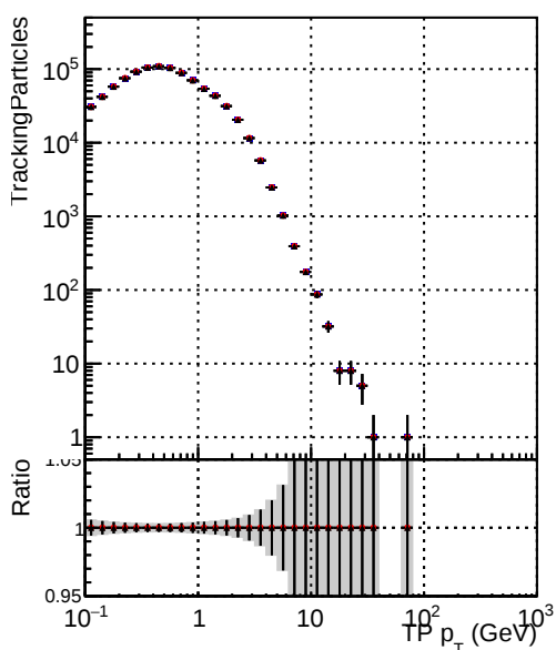
● DQM_CKF_SoftQCD ● DQM_mkFit_SoftQCD-noDNN-baseline ● DQM_mkFit_SoftQCD-noDNN-fix
