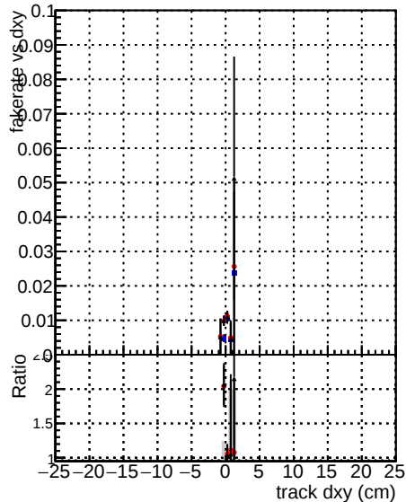
— DOM CKF SoftQCD — BSM-mkFit SoftQCD-noBNN-bx
