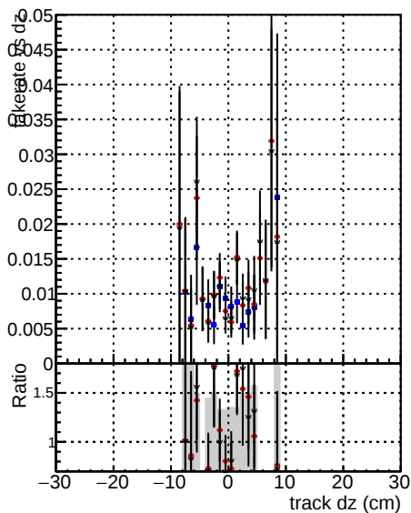
— DOM CKF SoftQCD — BSM-mkFit SoftQCD-noBNN-bx
