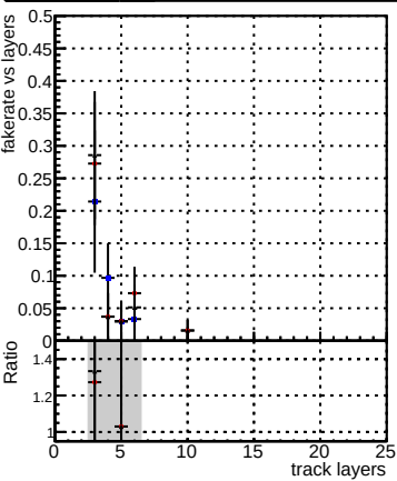
Legend: DQM_CKF_SoftQCD DQM_mkFit_SoftQCD-noDNN-baseline DQM_mkFit_SoftQCD-noDNN-fix
