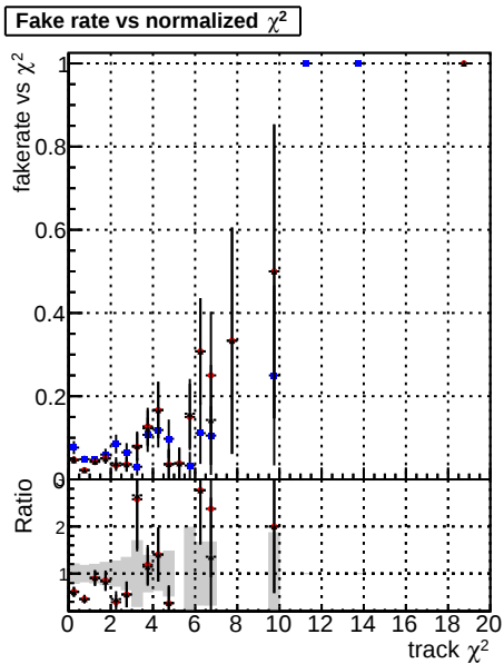
Fake rate vs. \chi^2 Legend: DOM, CKF, SoftOCB, SoftOCB-noDNN-fix
