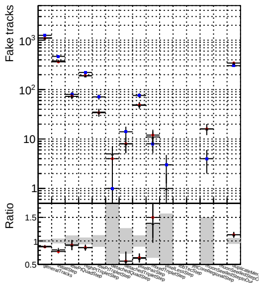
Number Legend 1 DQM_mkFit_SoftQCD-noDNN-baseline 2 DQM_mkFit_SoftQCD-noDNN-fix
