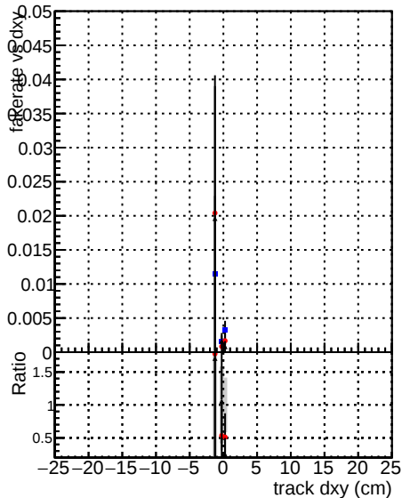
—•— DOM CKF SoftOCB —•— DOM mktFit SoftOCB-noDNN-baseline
