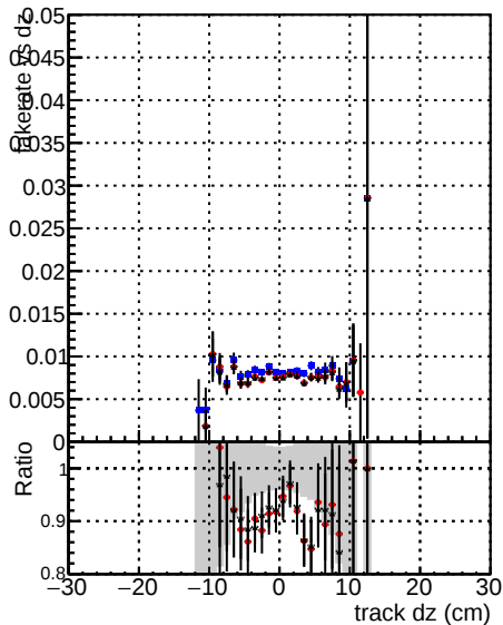
Fake rate vs dz DOM CKF SoftQCD DOM CKF SoftQCD-noBNN-fix
