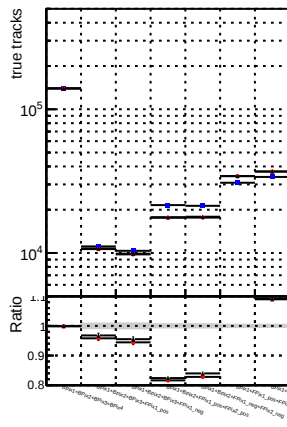
DOM CKF SoftOCD noDNN baseline N of reco track vs. s mkFit mkFit SoftOCD noDNN baseline mkFit mkFit SoftOCD noDNN fix
