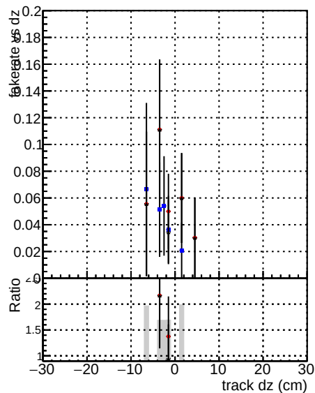
Fake rate vs dz Legend: DOM (black), CKF (blue), SoftOCB (red), SoftOCB-noBNN-fix (grey)
