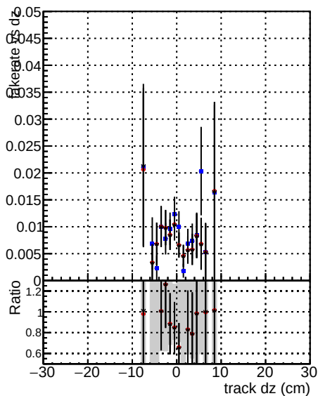
DOM CKF SoftQCD BNN-baseline DOM mktFit SoftQCD noBNN-fix
