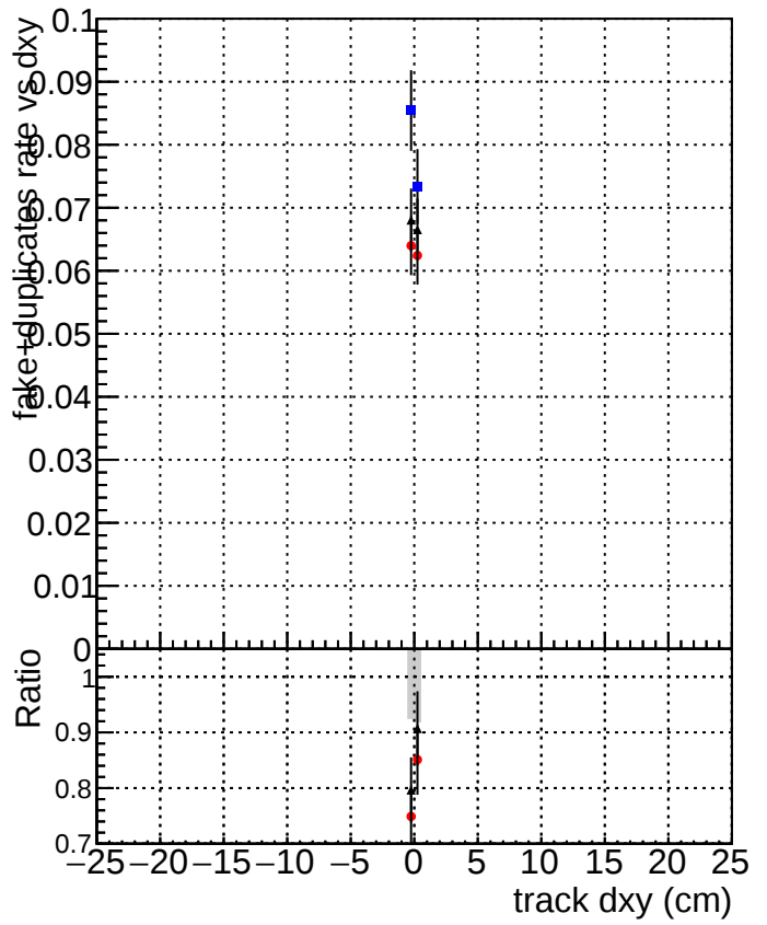
Legend: DQM_CKF_SoftQCD DQM_mkFit_SoftQCD-noDNN-baseline DQM_mkFit_SoftQCD-noDNN-fix
