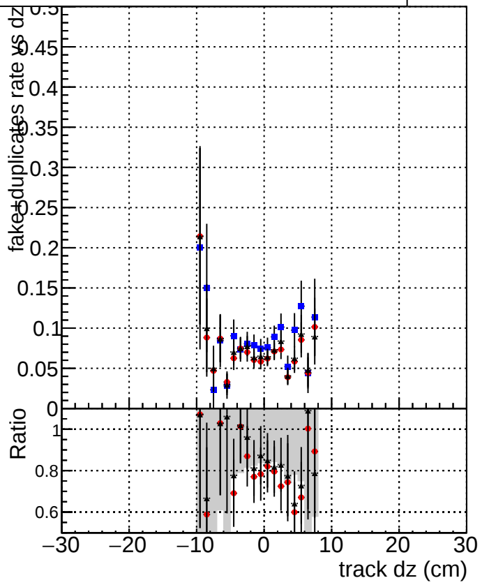
Legend: DQM_CKF_SoftQCD DQM_mkFit_SoftQCD-noDNN-baseline DQM_mkFit_SoftQCD-noDNN-fix
