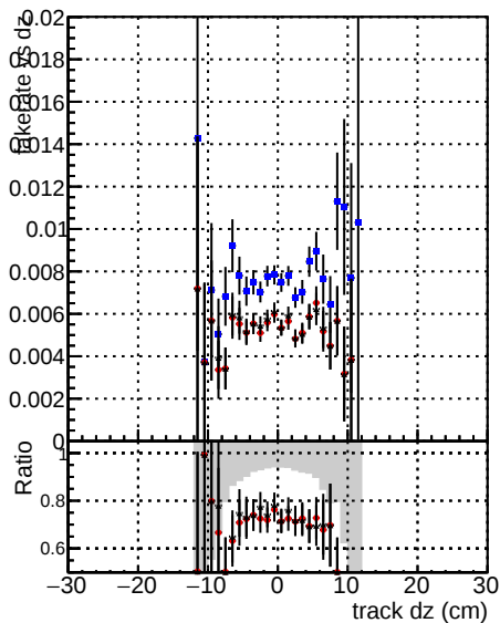
Fake rate vs dz DOM CKF SoftOCD DOM CKF SoftOCD-noBNN-fix
