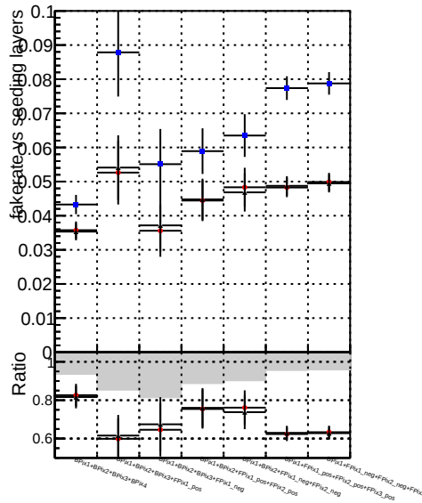
Fake rate vs. Legend: DOM, CKF, SoftOCB, BOM, mkt, SoftOCB-noBNN-baseline
