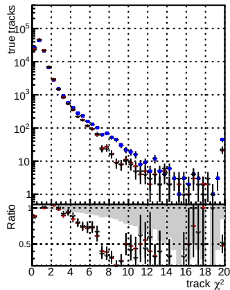
DBNN-baseline DBNN-fix
