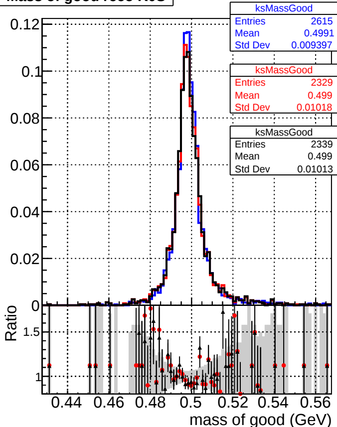
Mass of good reco K0S
