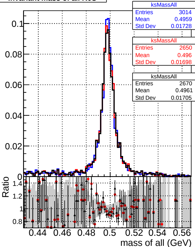
Invariant mass of all K0S
