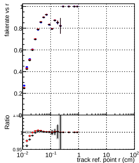
Fake rate vs vertpos — DOM_TTPU_mkFit_build (blue squares) — DOM_TTPU_mkFit_Fit (red circles) — DOM_TTPU_mkFit_100RescaleBoth (black crosses)
